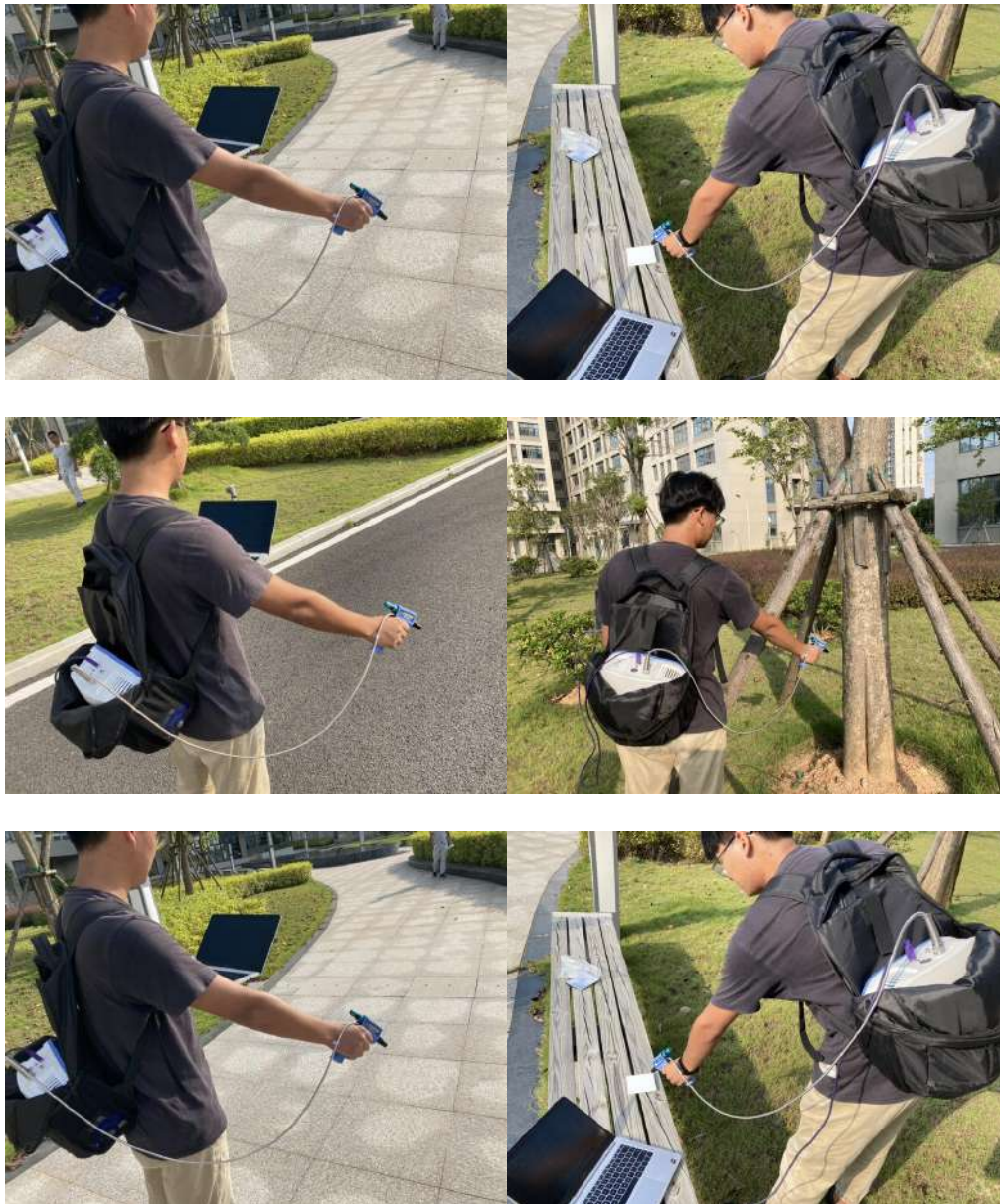
ATP9110 outdoor measurement pictures
